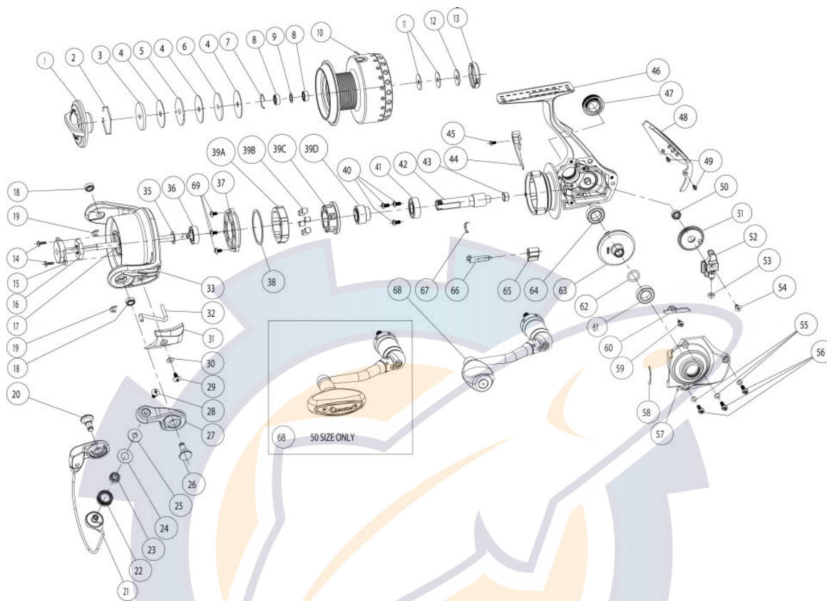
Quantum Catalyst Inshore CI40PTsB Spinning Reel Part List
